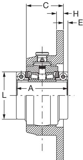
EXPANSION CONSTRUCTION
