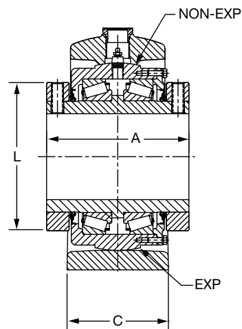
5-7/16" THRU 7" CONSTRUCTION
