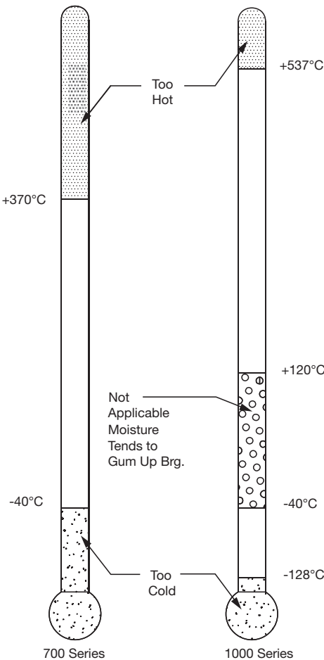
SOLIDLUBE Bearing Operating Temperature
