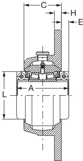
NON-EXPANSION CONSTRUCTION
