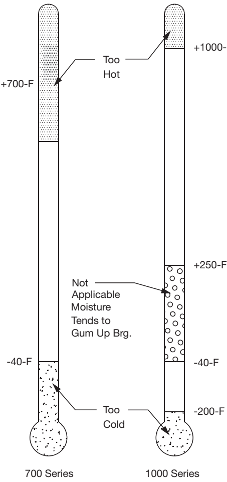
SOLIDLUBE Bearing Operating Temperature
