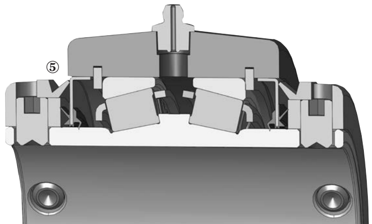
XTS Sealing with E-Test Option
