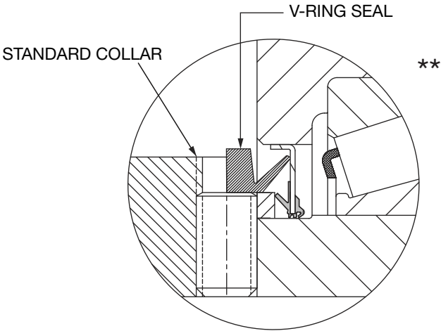
LARGE E-TECT SEAL 5-7/16 THRU 7"
