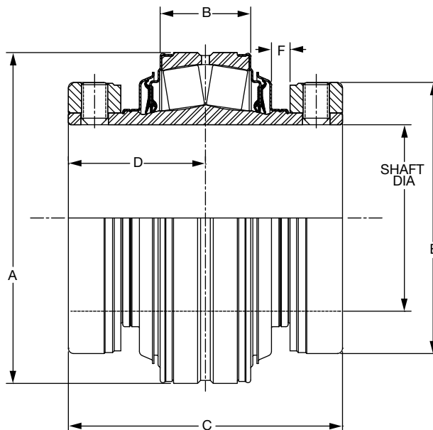
4-7/16 THRU 4-15/16" CONSTRUCTION
