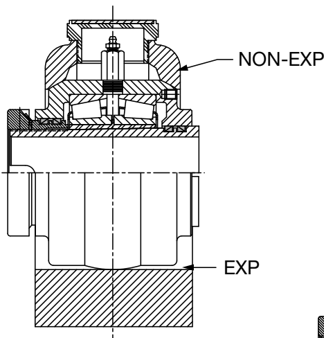
2-3/8" THRU 3-1/2" CONSTRUCTION
