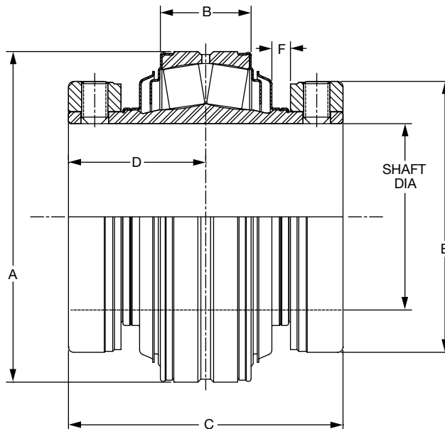
4-7/16 THRU 4-15/16" CONSTRUCTION
