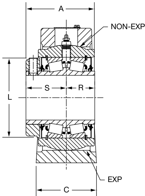
1-3/16" THRU 3" CONSTRUCTION
