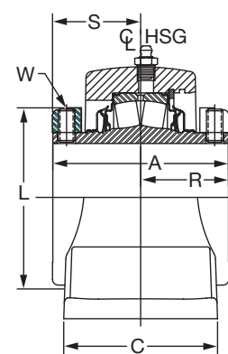
4-7/16 THRU 4-15/16" CONSTRUCTION
