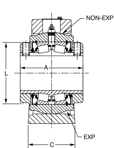
2-1/4" THRU 3" CONSTRUCTION
