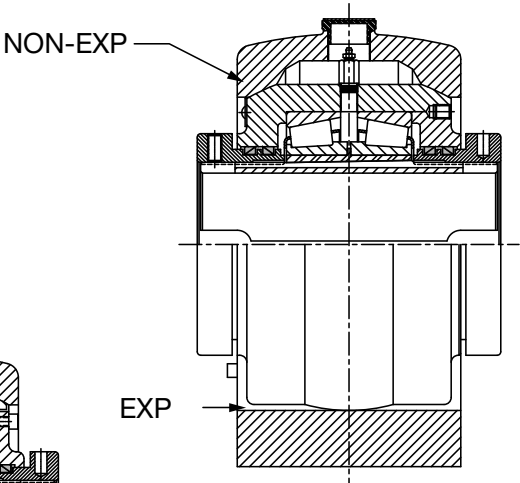
3-11/16" THRU 6" CONSTRUCTION
