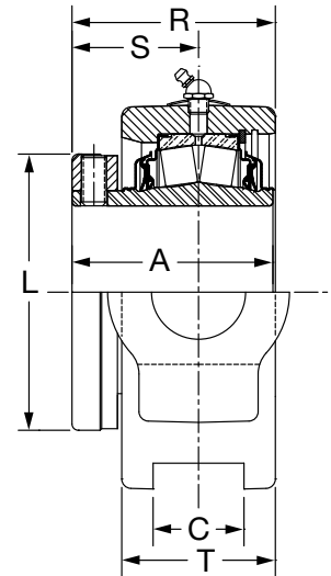
1-3/8 THRU 3-15/16" CONSTRUCTION
