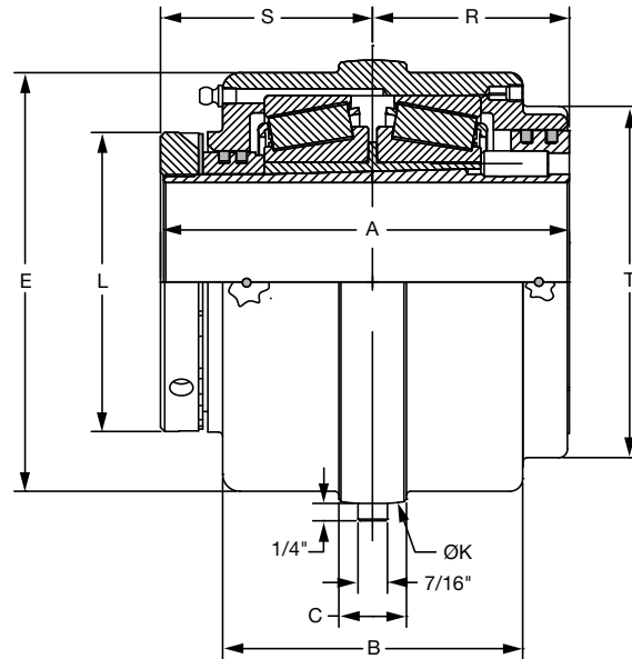
Hinged Cap Pillow Block S-1 Units
