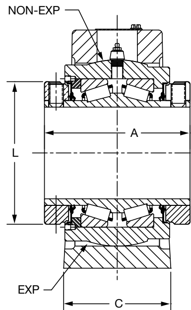
3-3/16" THRU 3-1/2" CONSTRUCTION
