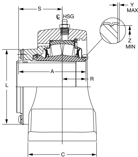
NON-EXPANSION
