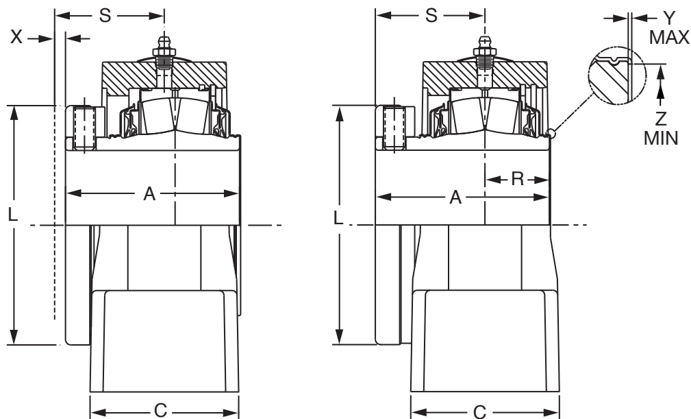
EXPANSION
