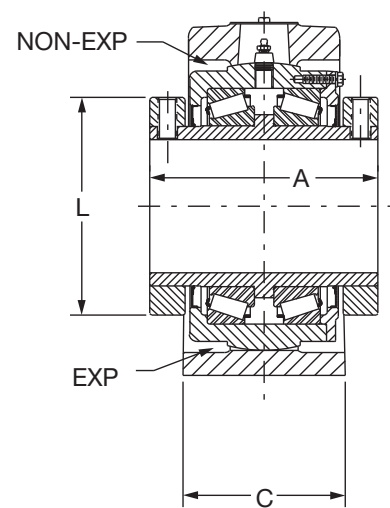
5-7/16" THRU 7" CONSTRUCTION
