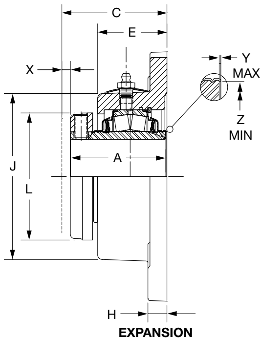
1-3/8" THRU 1-1/2" CONSTRUCTION
