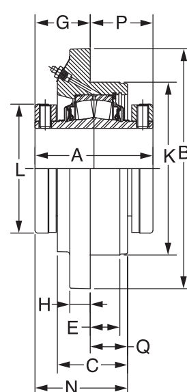
4-7/16 THRU 5" CONSTRUCTION NON-EXPANSION
