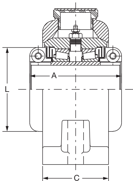
NON-EXPANSION CONSTRUCTION
