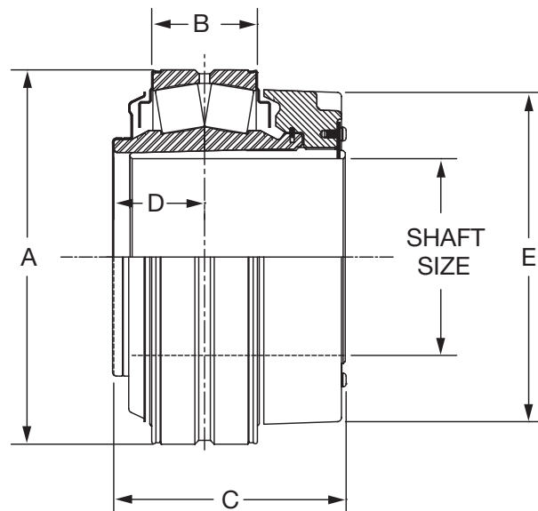
LABYRINTH SEAL
