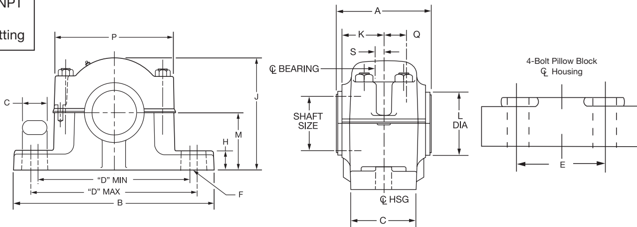
(22200K Adapter Mount Bearing)
