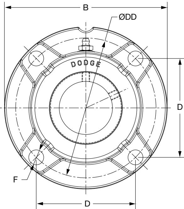
1-11/16" - 3" CONSTRUCTION
