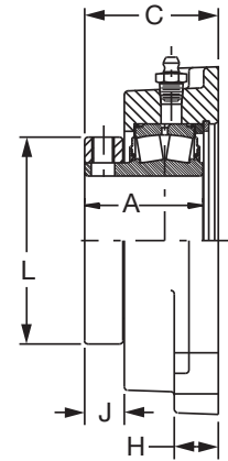
NON-EXPANSION
