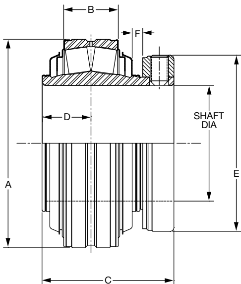
1-3/8 THRU 3-15/16" CONSTRUCTION
