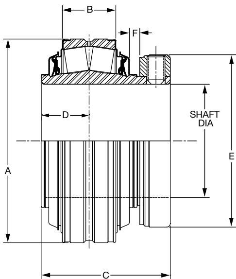
1-3/8 THRU 3-15/16" CONSTRUCTION
