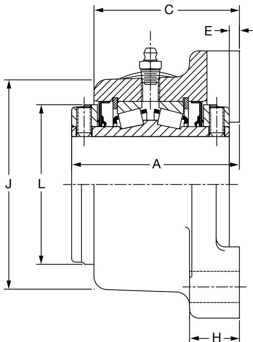
1-3/16" THRU 3" CONSTRUCTION
