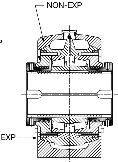
6-1/16" THRU 8" CONSTRUCTION
