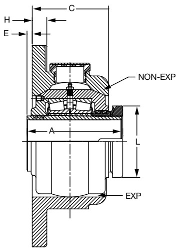
1-3/8" THRU 3-1/2" CONSTRUCTION
