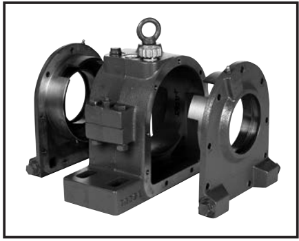
Split housing with bolt-on end covers
