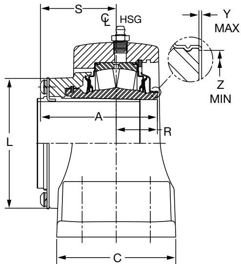
3-11/16" THRU 5" NON-EXPANSION
