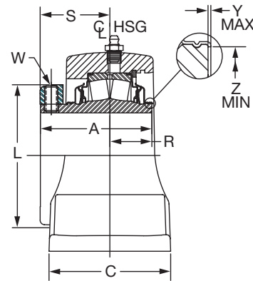
2-7/16 THRU 3-15/16" CONSTRUCTION
