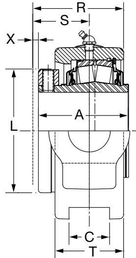
1-3/8 THRU 3-15/16" CONSTRUCTION
