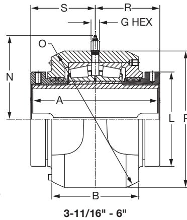
D-UNIT
