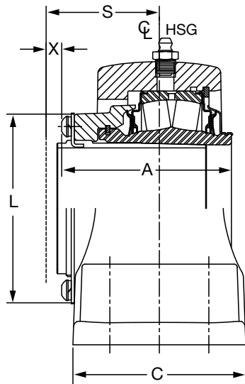
3-11/16" THRU 5" EXPANSION
