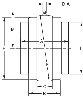
S-1 UNIT
