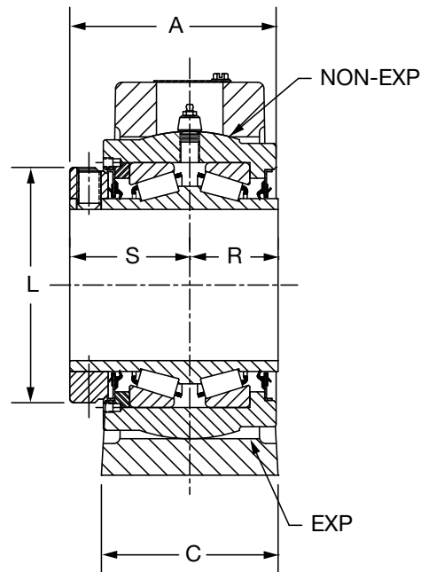
3-3/16" THRU 3-15/16" CONSTRUCTION
