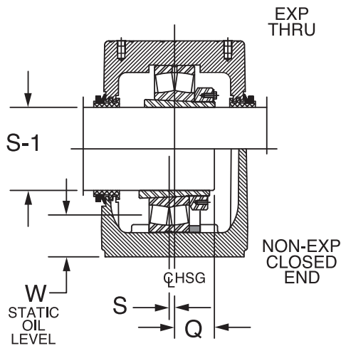
23000 SERIES (REQUIRES (1) STABILIZING RING)
