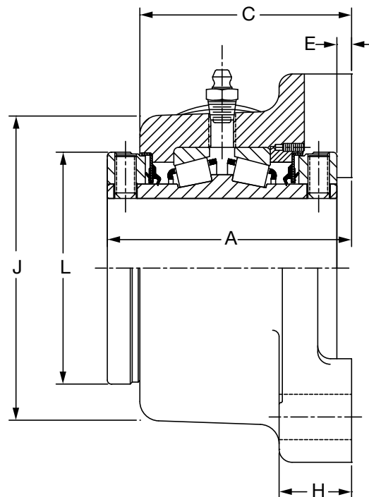
3-3/16" THRU 4-1/2" CONSTRUCTION
