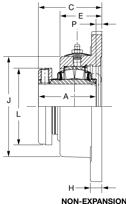
1-11/16" - 3" CONSTRUCTION
