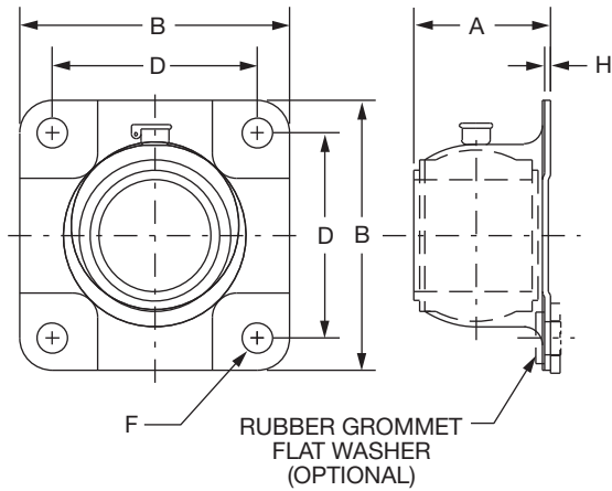
STYLE A
